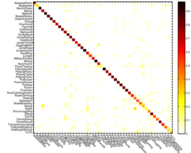
Fig. 8. Confusion matrix of ILRDFL on the UCF50 database. The classification rates are not shown. The color legend is drawn on the right, best viewed in color.
