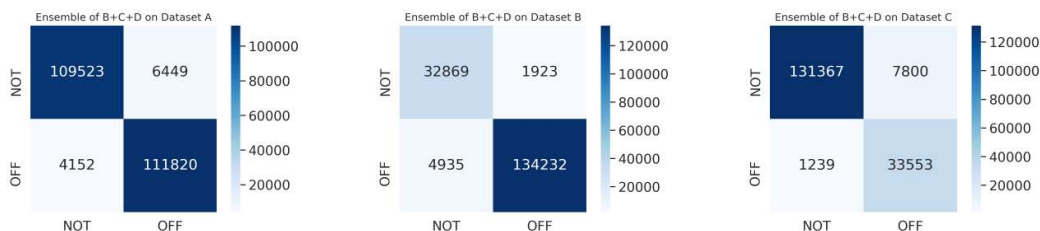
Figure 1: Confusion matrices of the best performing ensemble model for evaluation datasets A, B and C of subtask A
