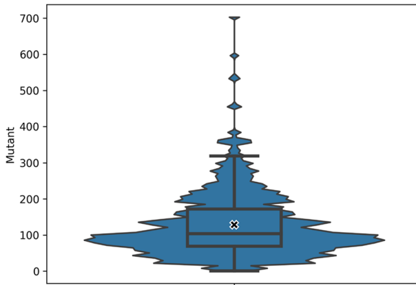
Fig. 3 Distribution of the number of generated mutants for Java input programs. The Y axis shows how many mutants were generated for the programs under test. Each data point represents a single program. The “X” marks the mean
