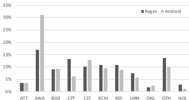
Fig. 3. Relative frequency of the assigned link purpose codes for both cases ( n_{regex} = 279 , n_{android} = 480 ).
