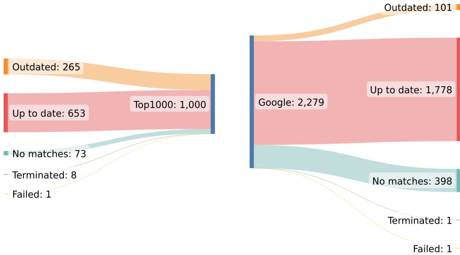
Fig. 5.1 Analysis status of top1000 and google projects, indicating whether a repository's documentation is currently out of date
