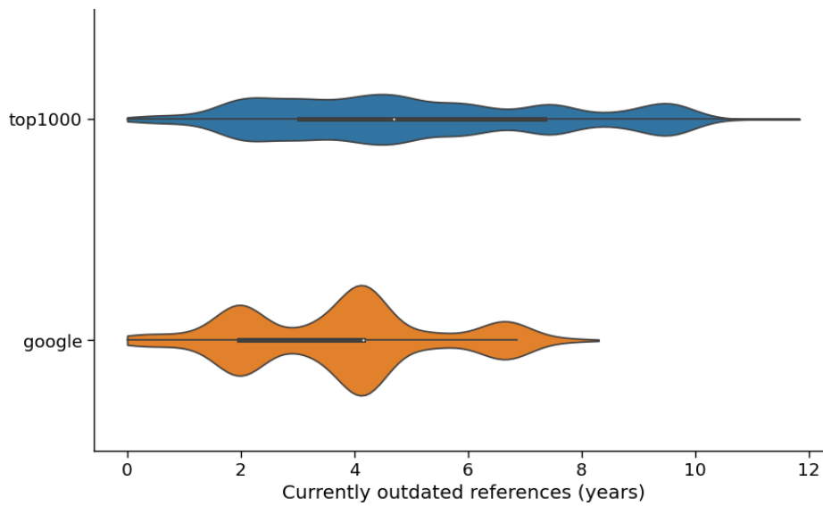
Fig. 5.3 Distribution of duration that code element references have been outdated for at the time of analysis in top1000 and google projects
