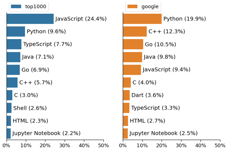
Fig. 3.2 Top 10 programming languages used in top1000 and google projects
