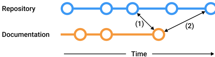
Fig. 3.3 Linking the current documentation version to (1) repository snapshot and (2) current repository revision
