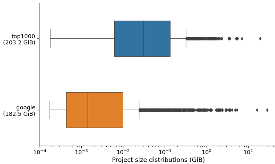
Fig. 3.1 Project size distributions (GiB) for top1000 and google projects in log scale
