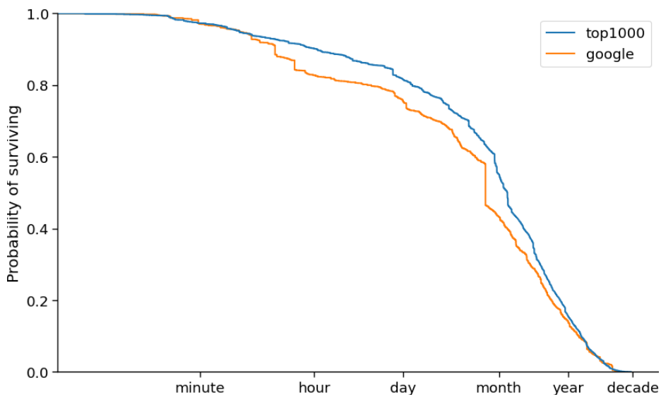
Fig. 5.6 Time taken to fix outdated references in documentation for the top1000 and google dataset in log scale
