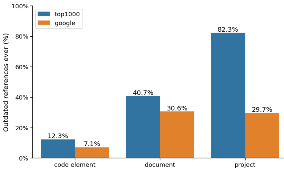
Fig. 5.4 Percentage of references outdated at least once at some point during its history on code element, document and project levels
