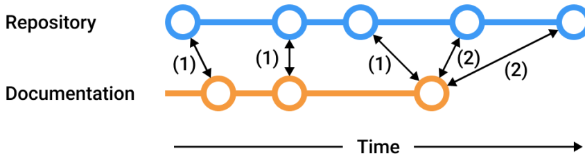
Fig. 3.4 Linking each repository revision to a corresponding documentation version for repository commits made (1) before and (2) after the current documentation version
