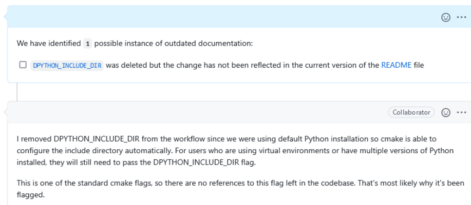
Fig. 5.9 False positive: still relevant for users with multiple Python versions
