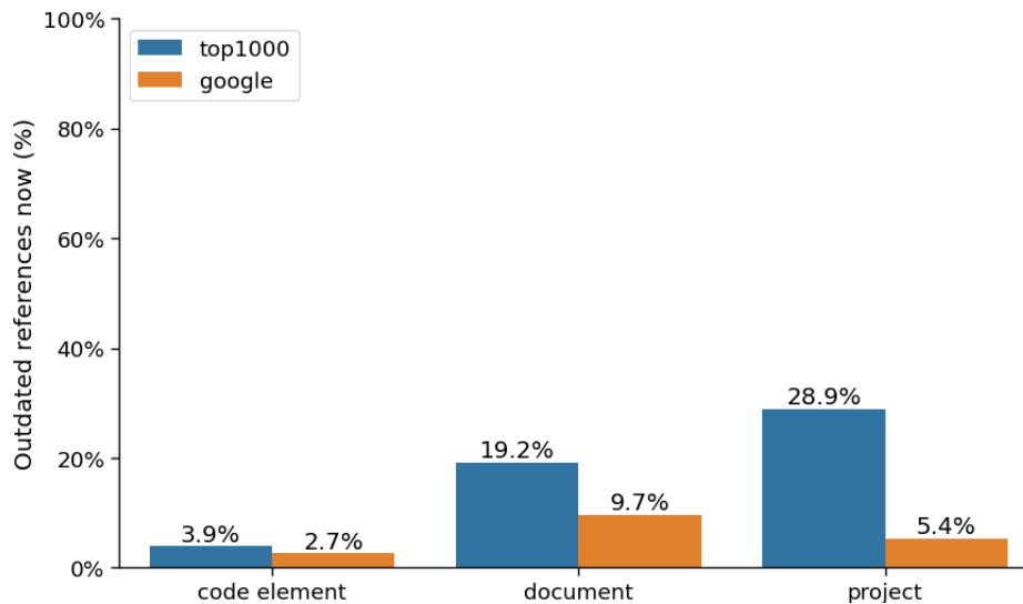
Fig. 5.2 Percentage of references outdated at the time of analysis on code element, document and project levels
