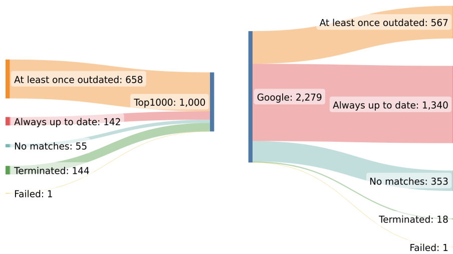
Fig. 5.5 Extended analysis status of top1000 and google projects, indicating whether a repository’s documentation was outdated at some point during its history
