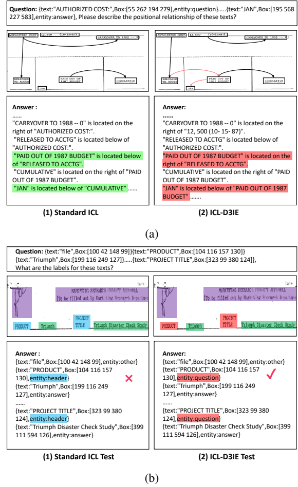
Figure 6: Case study on comparison of (a) positional relationship description and (b) predictions generated by Standard ICL (Davinci-003) and ICL-D3IE (Davinci-003).
