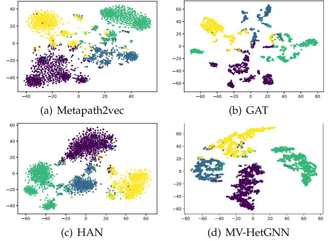
Fig. 6. Visualization of embeddings on DBLP. Each point denotes one author and its color indicates the research area.
