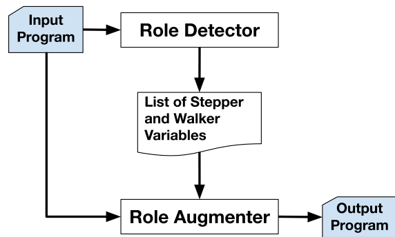
Fig. 1: Role detection and augmentation workflow.
