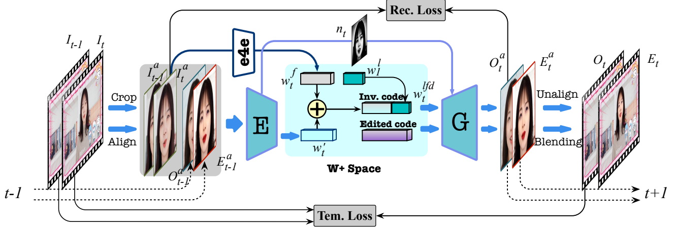
Figure 2: Overview of our RIGID. We first align the faces on two neighbor frames ( I_{t-1} and I_t ). Then we concatenate them with the inverted face O_{t-1} and edited face E_{t-1} in the previous step as the inputs of the recurrent encoder. The encoder learns the temporal compensated code w_t^f and spatial noise map n_t , as a complement to the initial latent code w_t (acquired by the “e4e” encoder). In addition, we share the latter part of latent codes across all frames using w_t^l for eliminating the high-frequency temporal flickering. Both the final inverted latent code w_t^{lfid} and the edited one are fed to the generator, producing the inverted and edited faces O_t^a and E_t^a . The generated faces are unaligned and blended with the original frames. Dotted lines denote recurrent inputs from the last time step or outputs to the next step. In addition, a novel in-between frame composition constraint is proposed that learns the temporal correlation during editing (details can be found in Fig. 3).
