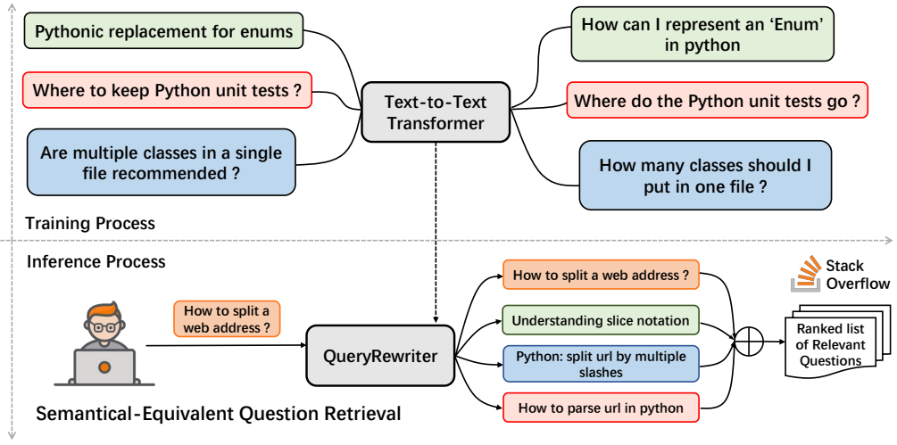
Fig. 3. QueryRewriter Workflow
