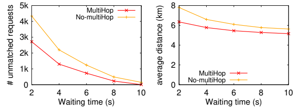
(a) # unmatched requests. (b) Average trip distance. Figure 11: Effect of the waiting time.
