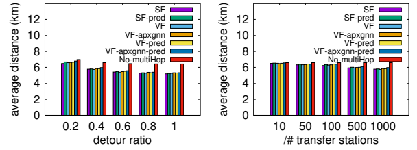
(a) Effect of the detour ratio. (b) Effect of the # transfer points. Figure 10: Average trip distance.
