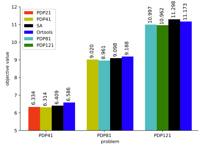
Fig. 5: Generalization on larger problem size.
