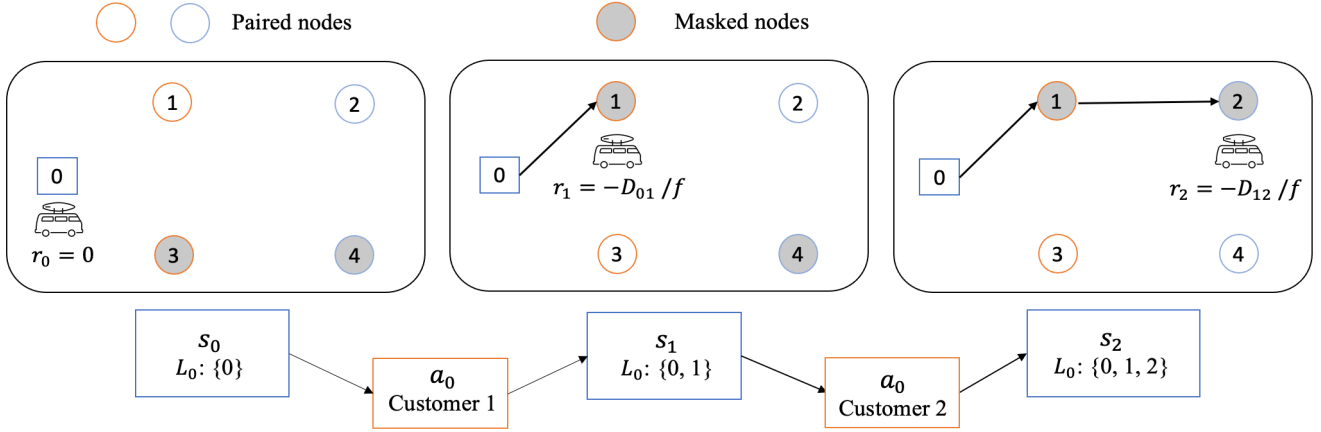
Fig. 1: An illustrative example of MDP with 1 vehicle and 4 nodes. Node x_1 and x_2 are pickup nodes, and node x_3 and x_4 are their delivery nodes, where node x_1 and x_3 , node x_2 and x_4 are paired. At the beginning, node x_3 and node x_4 are masked due to the precedence constraint. At the first step, node x_1 is selected, i.e., a_1 = x_1 . In response to this action, a) node x_1 is masked and node x_3 becomes unmasked; b) the partial route is updated, i.e., L_1 = \{0, 1\} ; c) the accumulative reward for this step is the negative value of the travel time of the vehicle travelling from the depot to node x_1 , i.e., r_1 = -D_{01}/f . At the second step, node x_2 is selected, and the state, action, reward are updated similarly.
