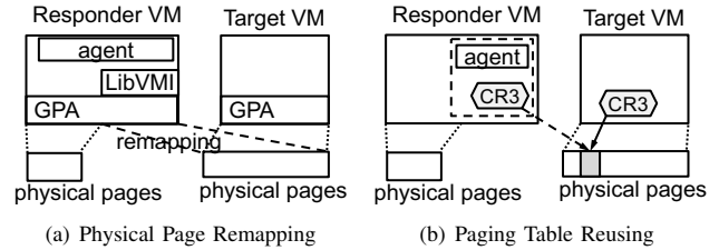
Fig. 2. Illustration of two difference methods of providing target mappings to the tool in the Responder VM.
