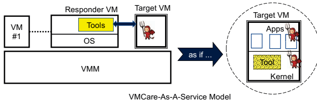
Fig. 1. Illustration of VMCare-As-A-Service. The target VM is undependable due to attacks subverting the kernel.
