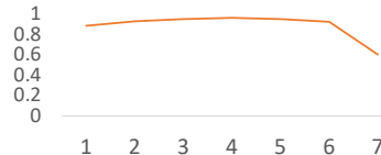
Fig. 3. Recall@1 (y-axis) versus like number (x-axis) within a maximum of 7 iteration rounds on MSR-VTT.
