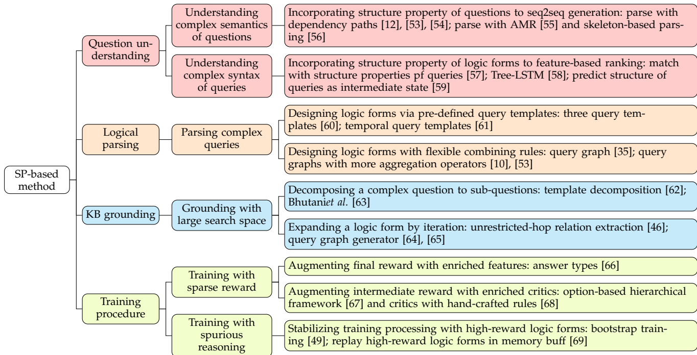
FIGURE 4: The main content of SP-based methods. The hierarchical structure is arranged with: SP-based method \rightarrow module \rightarrow challenge \rightarrow solution.
