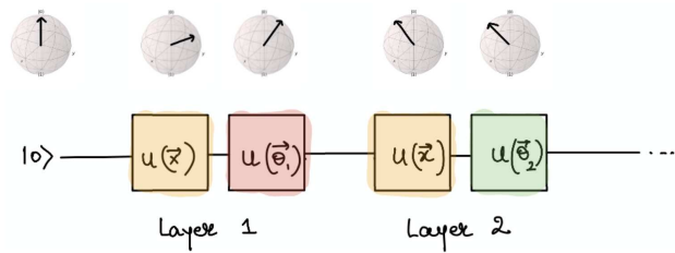
Figure 9. Quantum circuit implementing data re-uploading, each block corresponds to the layer of classical neural network. Image is taken from the online source Ref. 53 .
