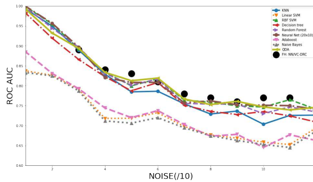
Figure 5. ROC/AUC for increasing level of noise for the classification of 2d dataset. Here we benchmark a great number of classical classifiers against our proposed FULL HYBRID classifier.
