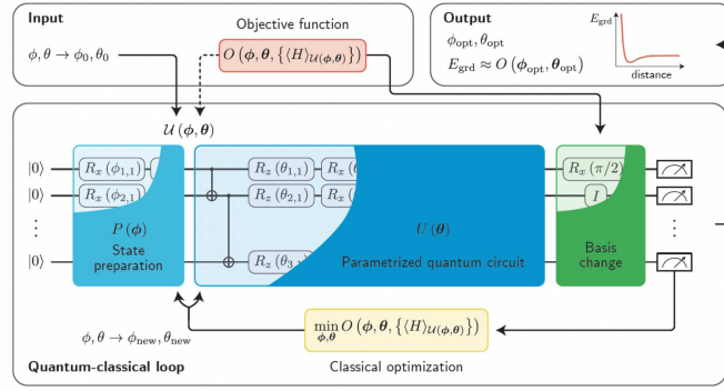
Figure 8. Schematic diagram of a Variational Quantum Algorithm (VQA). Figure is taken from the Ref. 2 .
