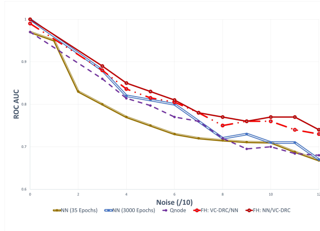
Figure 4. ROC/AUC for increasing level of noise for the classification of 2d dataset. Here we benchmark FH versus just the classical part (NN) and versus just the quantum part (Qnode).
