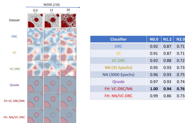
Figure 6. (Right) ROC/AUC for classifiers for different noise levels. (Left) Prediction grids for respective classifiers for different noise levels.
