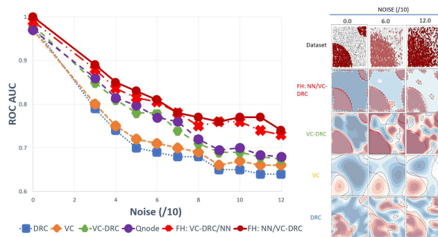
Figure 3. (Left) ROC/AUC for DRC, VC and VC-DRC classifiers for different noise levels. (Right) Prediction grids for respective classifiers for different noise levels.
