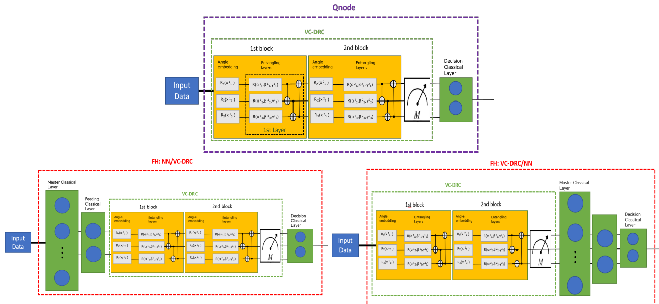
Figure 12. (First row) Block Diagram of the specific QNode proposed in the current study. (Second row) Block Diagram of the Full Hybrid (NN/VC-DRC) classifier where a VC-DRC circuit is placed after a classical neural network, (Third row) Block Diagram of the Full Hybrid classifier where a fully quantum VC-DRC circuit is placed before classical neural network (VC-DRC/NN).
