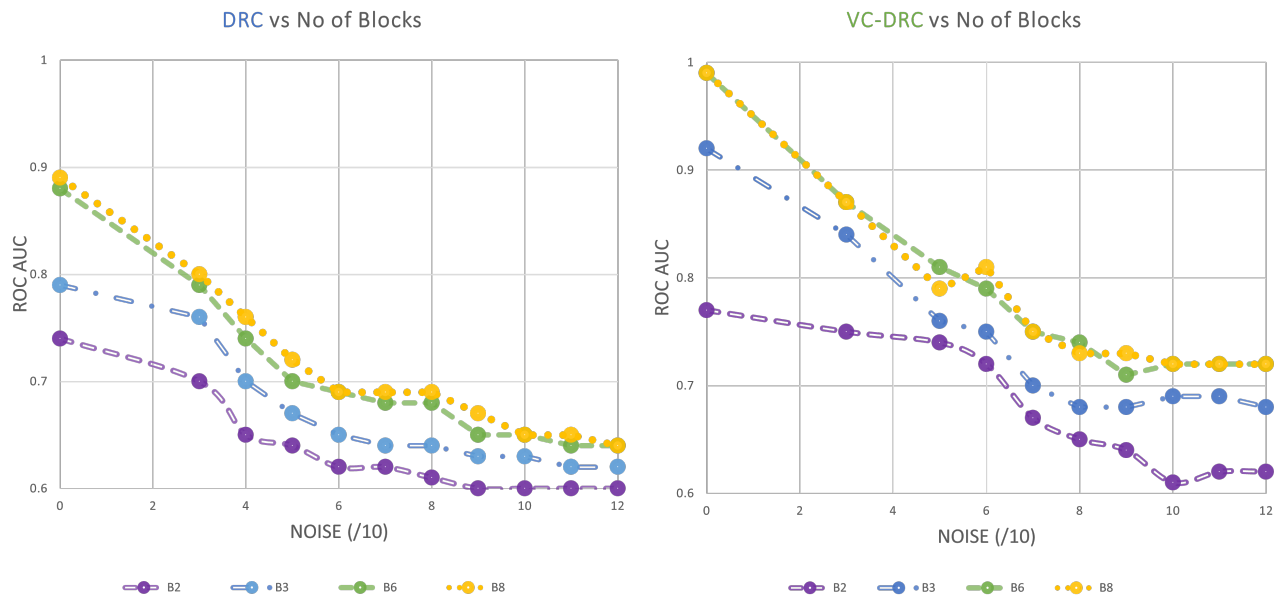
Figure 2. ROC/AUC as a function of number of repeating blocks of data re-uploading for the DRC classifier (left) and VC-DRC classifier (right)
