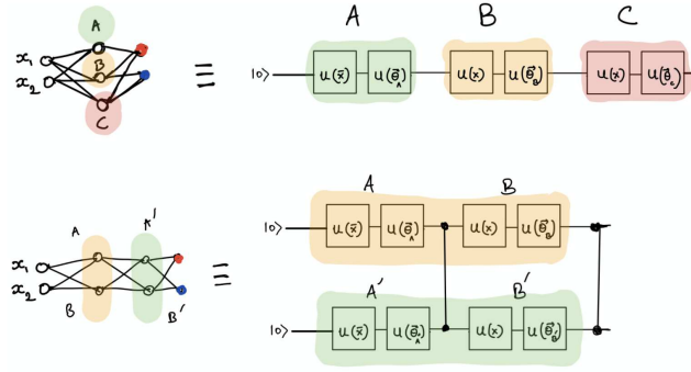
Figure 10. Quantum circuit implementing data-reuploading with strongly entangling layers, where entanglement between the blocks is introduced with controlled two-qubit gates. Figure is taken from the online source Ref. 53 .
