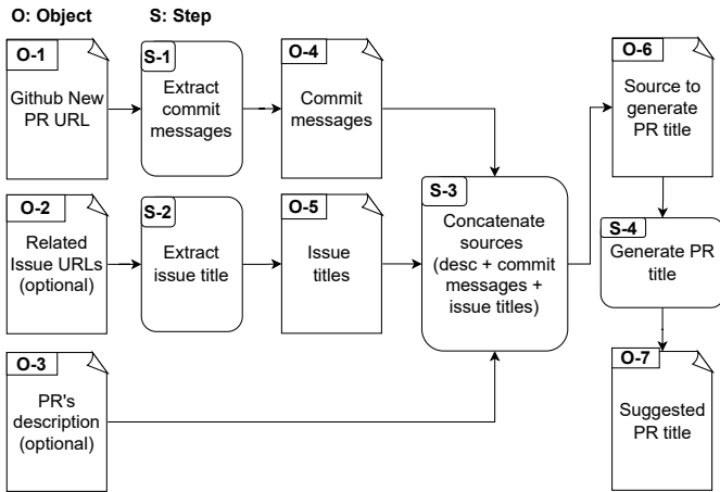
Fig. 1. The architecture of AUTOPRTITLE
