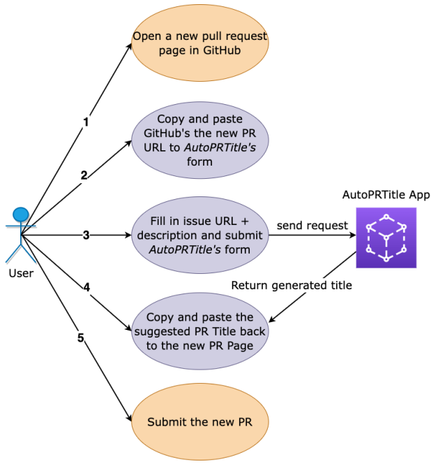
Fig. 3. The scenario of using AUTOPTITLE
