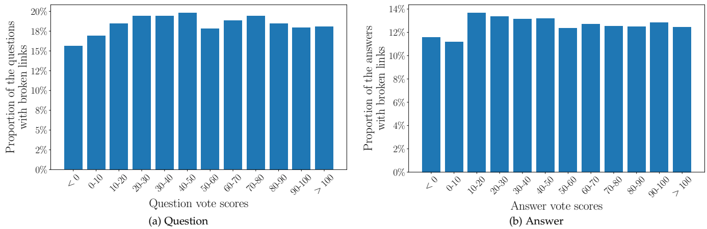
Fig. 5: The proportions of the broken posts among the posts with links based on the vote scores. These figures show that broken links are common across questions and answers with different vote scores.
