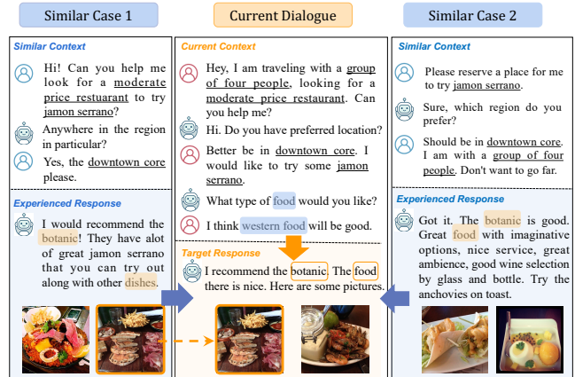
Figure 1: Example dialogue for venue recommendation, where two similar cases provide useful guidance.
