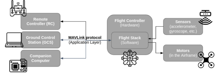
Fig. 1: A typical drone system
