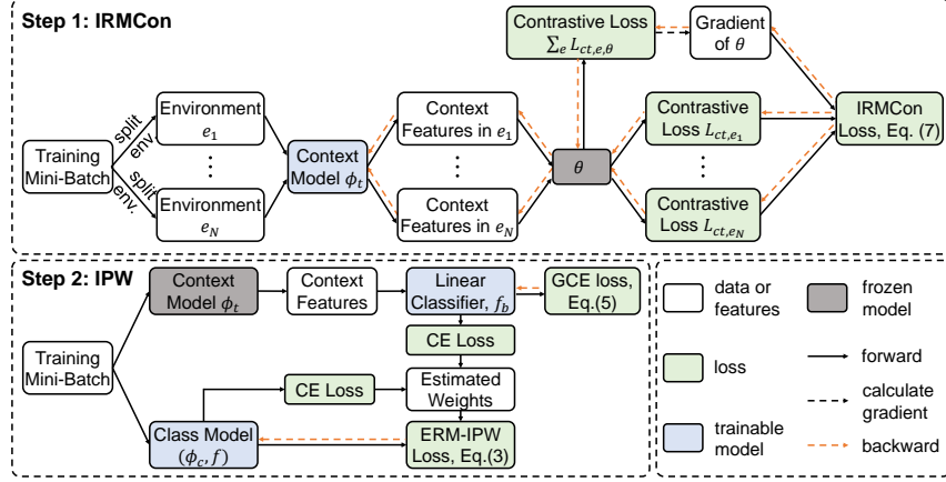
Fig. 3. The training pipeline of our IRMCon-IPW. 1) “split env.” denotes we split the training samples in mini-batch into subsets based on class labels, i.e., samples of each class in one subset, forming N environments \{e_i\}_1^N ; 2) \theta is a dummy classifier, whose gradient is for regularizing \phi_t become invariant to classes. See the detailed algorithm in Appendix
