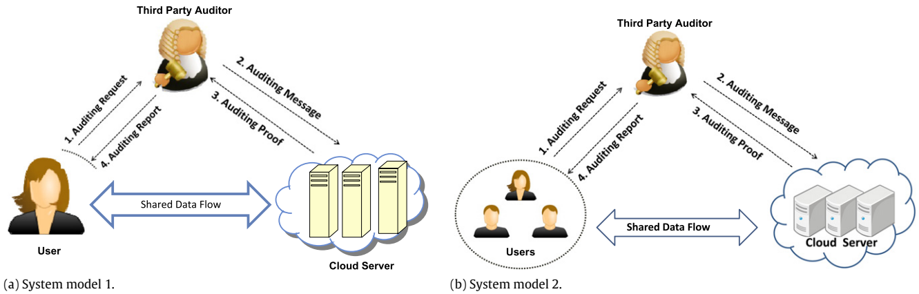
Fig. 1. The system model of auditing mechanisms for secure cloud storage.
