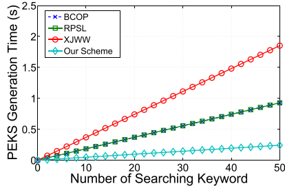
Fig. 7. Computation cost of PEKS generation in different schemes.
