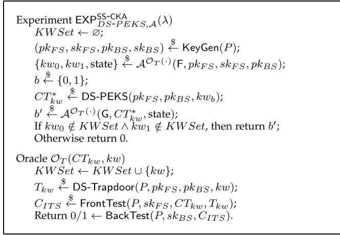
Fig. 1. SS-CKA experiment for adversarial front server.
