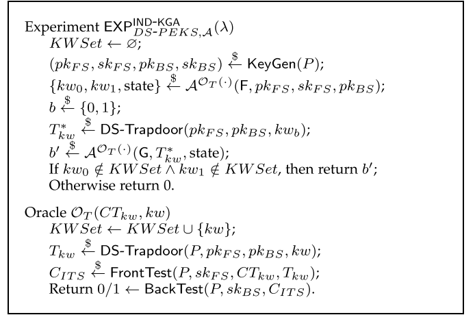
Fig. 2. IND-KGA experiment for adversarial front server.
