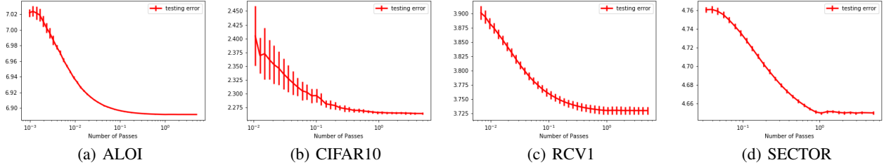
Figure 1: Testing errors versus the number of passes.
