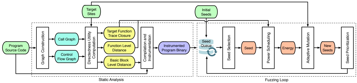
Figure 3: Approach Overview of Hawkeye
