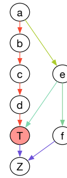
Figure 2: The fuzzing scenario modeled from Fig. 1: \langle a, b, c, d, T, Z \rangle is a crashing trace passing T , \langle a, e, T, Z \rangle is a normal trace passing T , and \langle a, e, f, Z \rangle is a trace not passing T .
