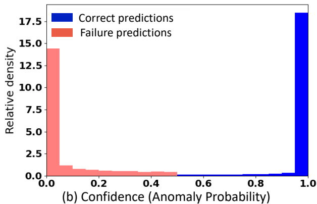
Fig. 3. Comparison of confidence learning based on (a) the prediction probability and (b) anomaly probability for failure prediction on the validation set of X-VIRAL.
