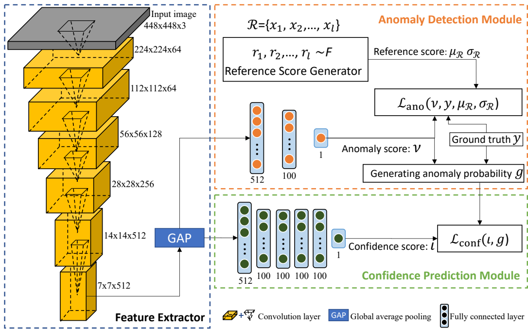
Fig. 2. Diagram of the proposed CAAD model. This model is composed of an anomaly detection module and a confidence prediction module, which are designed to predict the anomaly score and confidence score of each input, respectively.
