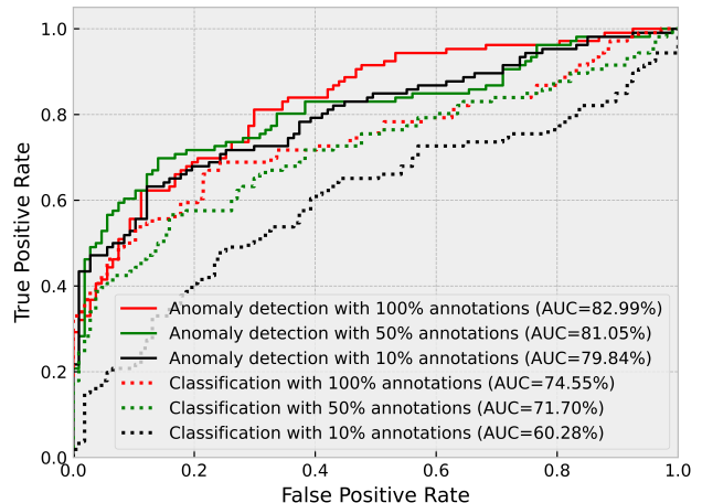
Fig. 7. AUC curves of anomaly detection and binary classification models obtained on X-COVID when both models were trained on X-VIRAL using all negative samples and 100%, 50%, and 10% positive samples, respectively.
