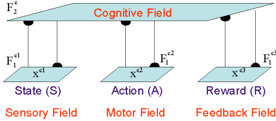
Fig. 1. TD-FALCON architecture.
