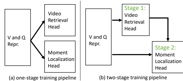
Figure 1: Comparisons between one-stage and two-stage training pipeline. V and Q Repr. means the video and query representations extracted from the backbone. One-stage training pipeline uses a model to train a video retrieval head and a moment localization head simultaneously whereas two-stage training pipeline uses the first model to train a video retrieval head and the second model to train a moment localization head.
