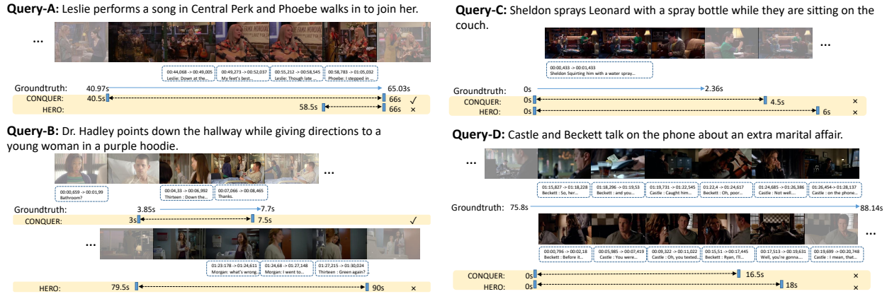
Figure 3: Four example queries showing the moments localized by CONQUER and HERO. A tick is given to the correctly localized moment, while a cross indicates negative localization because of IoU \leq 0.7 . Best view by zooming to cross-read the query, subtitle and video timeline.
