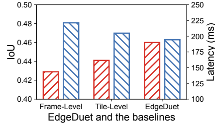
Fig. 14. Benefits of Content-Prioritized Tile Offloading
