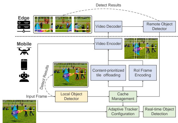
Fig. 2. An overview of EdgeDuet. Rectangles in different colors represent the three functional modules (offloaded small object detection (blue) (Sec. III), local object detector (yellow) (Sec. IV) and real-time tracking (green) (Sec. V). EdgeDuet is implemented as a cross-platform framework consisting of both edge-side and device-side modules (Sec. VI).
