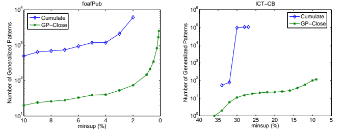
Figure 3: Number of patterns extracted by GP-Close compared with Cumulate.
