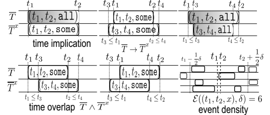
Fig. 5. Different kinds of temporal relations.
