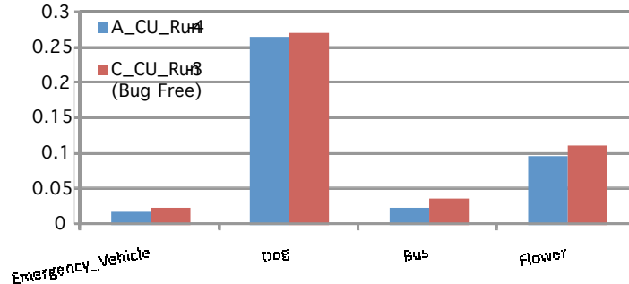
Figure 4: Performance improvement by adding additional training images from the Web. Note that Run-3 is generated by fusing Run-4 with another SVM classifier trained from web images (see Section 1.4 for more details).
