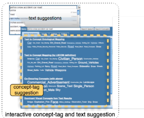
Figure 7: The query formulation panel provides users with textual word-completion and a set of relevant concepts via numerous suggestion methods (figure from [1]).
