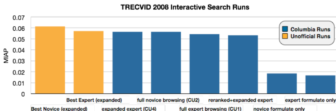
Figure 9: Performance of best CU runs compared to official TRECVID2008 submissions.
