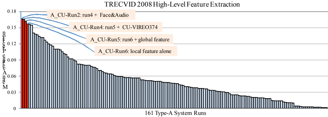
Figure 3: Performances of our submitted type-A runs and all 161 official type-A HLF submissions.
