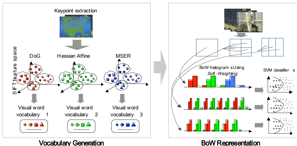
Figure 2: Framework of our local feature representation.
