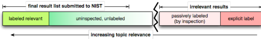
Figure 6: Typical result ordering for formulating final results list for TRECVID evaluation.
