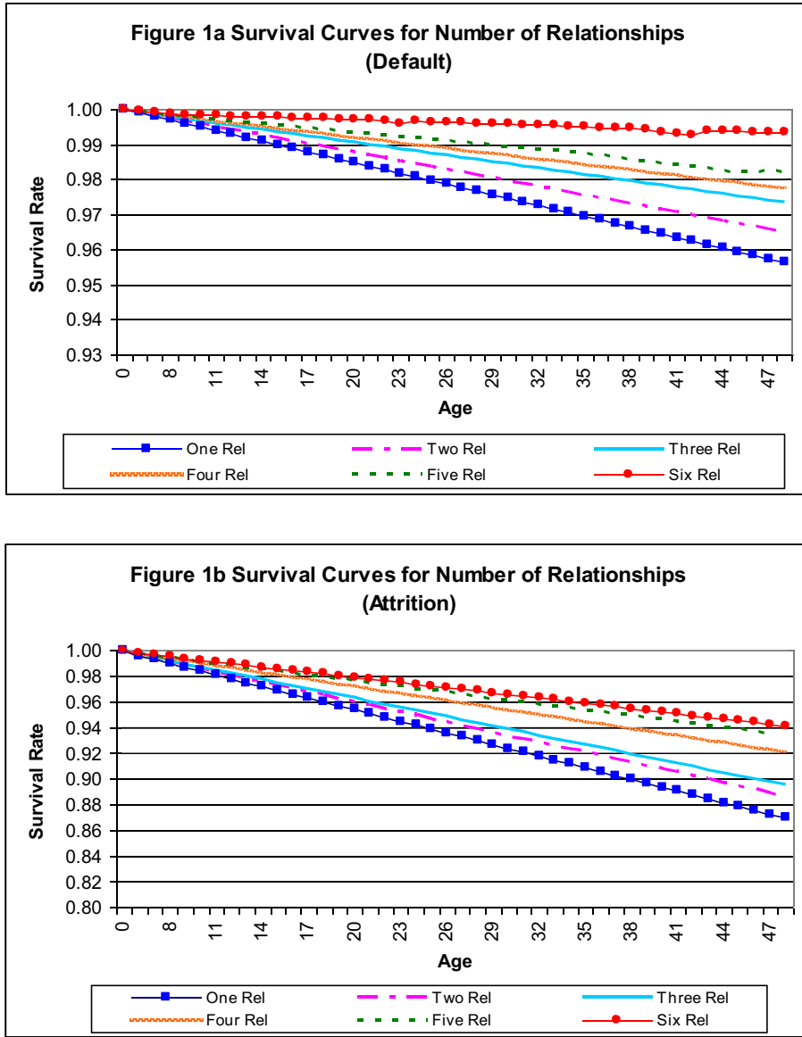
Fig. 1. Survival curves for different numbers of relationships.
