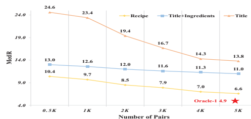
Figure 5: Performance trend with increasing number of pairing information available for linking text and image modalities (Chuan→Washoku). The performance of Oracle-1 is indicated with asterisk for reference.
