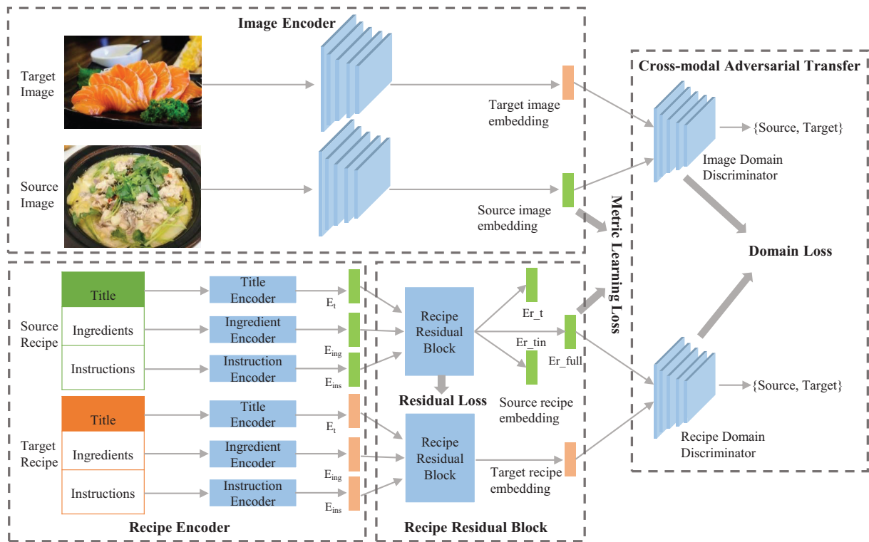
Figure 1: The architecture of cross-domain food transfer.
