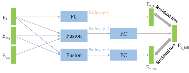
Figure 2: The architecture of Recipe Residual Block.
