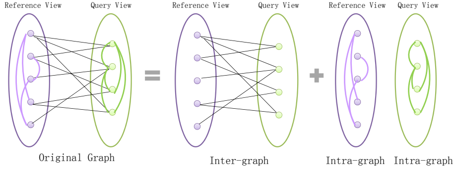
Fig. 1. Illustration of Cross-view Graph Embedding: the original graph could be divided into one inter-graph which is a bipartite graph and two intra-graphs.
