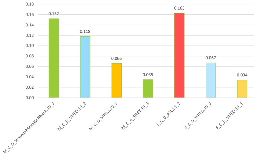
Figure 2: Performance comparison of official auto and manual runs.
