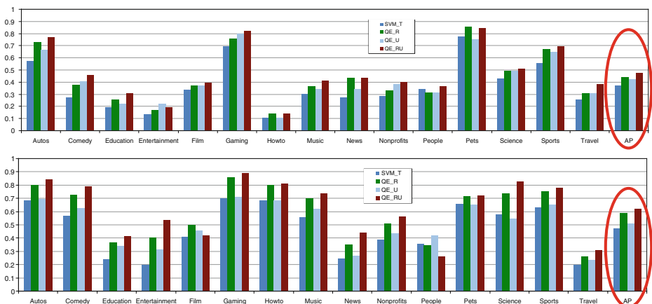
Figure 5 Performance comparison for query expansion on TS_A (upper part) and TS_B (lower part) datasets.
