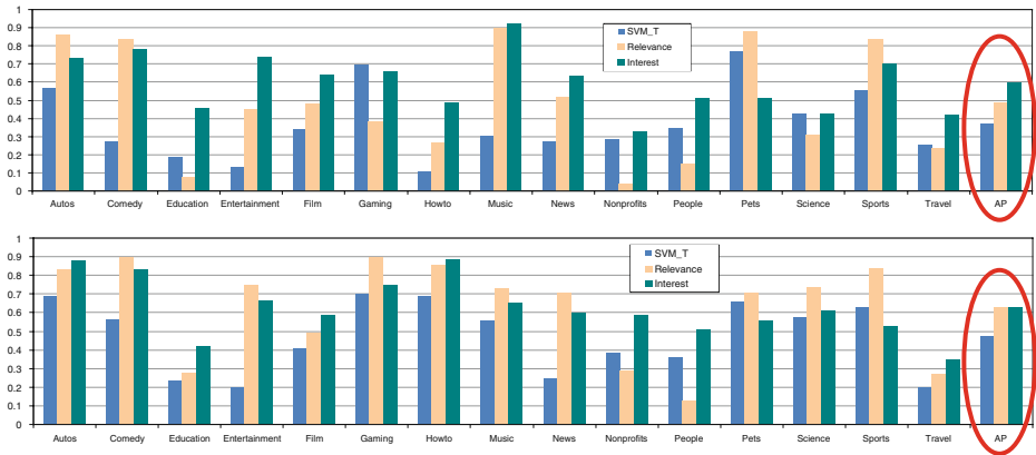
Figure 4 Performance comparison for model-based and data-driven approaches on TS_A (upper part) and TS_B (lower part) datasets.
