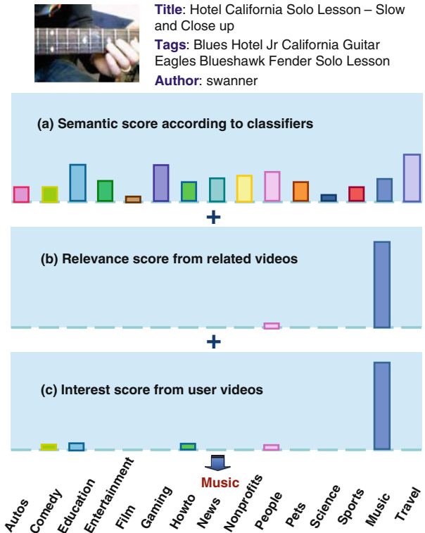
Figure 3 According to classifiers built on text (a), a video on guitar lesson is falsely suggested as “Travel” category. When considering video relevance (b) and user interest (c), it is correctly recommended as “Music” category.
