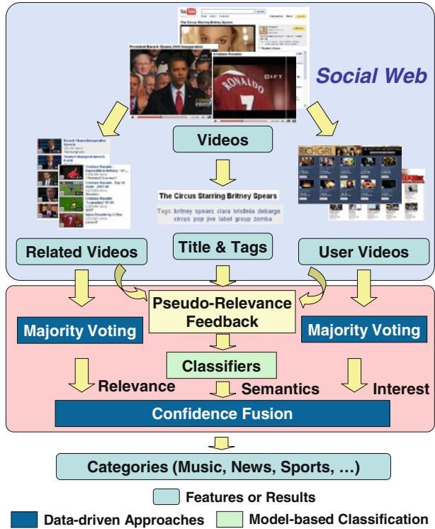
Figure 2 The framework of web video categorization.
