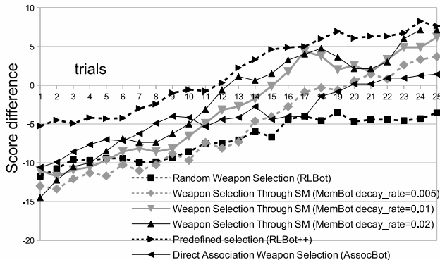
Figure 7: Performance of RLBot , RLBot++ , MemBot , AssocBot over 25 trials
