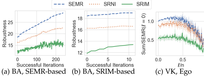
Fig. 15: Effect of rewiring (a,b), node removals (c)
