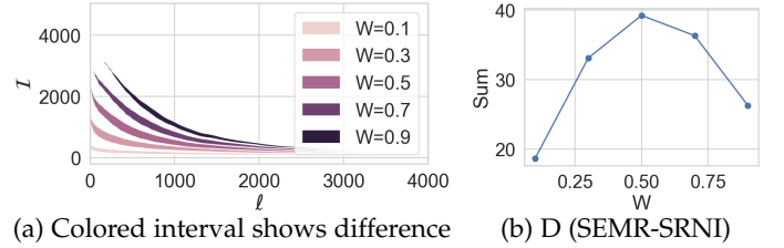
Fig. 13: D on DBLP. \alpha = 1.075 , k=50 , \beta=40 , Random .
