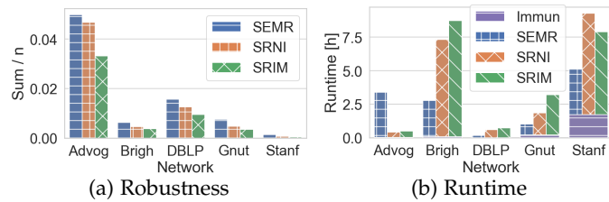
Fig. 19: Scalability on larger networks. W = 0.5 , Random , k = 100 , \alpha = 1.075 ; on Stanford: W = 0.1 , \alpha = 1.2
