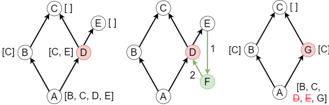
(a) A condensation (b) Adding node (c) Updating labels Fig. 1: Maintaining the DAG reachability index.
