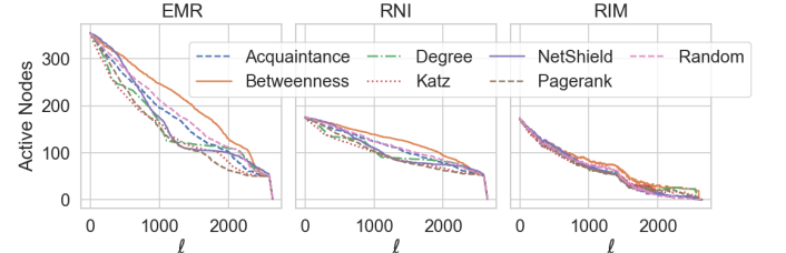
Fig. 5: Minnesota, 7 attack strategies, W=0.5 , k=50 , Random .
