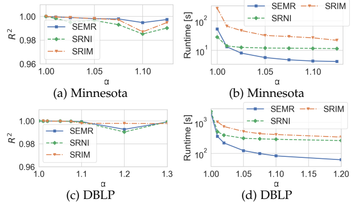
Fig. 17: Performance vs. \alpha ; R^2 averaged over adversaries, Random prob; Minnesota W = 0.7, k = 10 ; DBLP W = 0.5, k = 50 ; immunization time 2s on Minnesota, 82s on DBLP.
