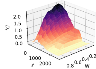
Fig. 10: IC, D_r , Minnesota, k = 10
