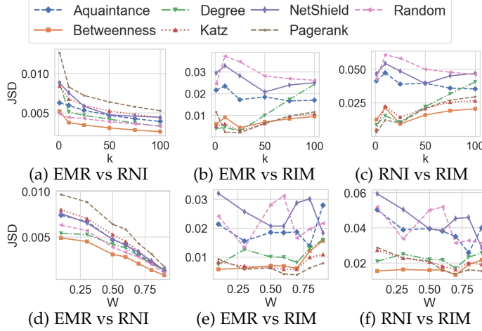
Fig. 6: JS divergence of measures per strategy.
