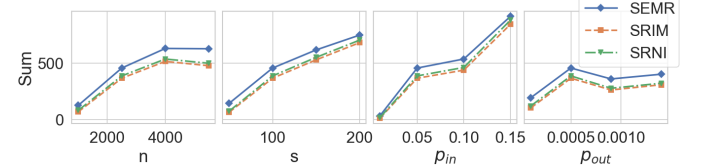
Fig. 9: Dependency on network parameters. GRP. n=2500 , s=100 , p_{in}=0.05 , p_{out}=5 \cdot 10^{-4} , k=10 , W=0.3 , Random .
