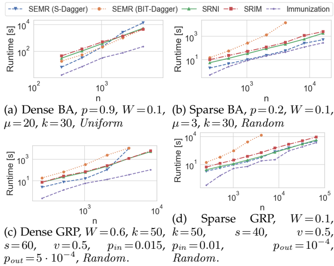
Fig. 18: Scalability on synthetic networks. \alpha = 1.075 .
