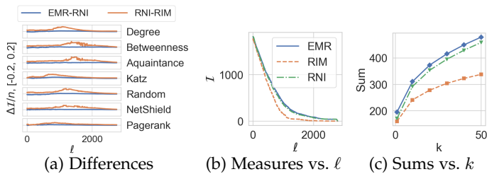
Fig. 7: Dependency of measures on VK social network.
