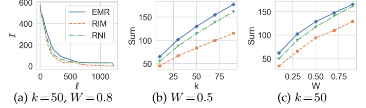
Fig. 8: Measures vs. \ell , k , W , Blogs network. Random .
