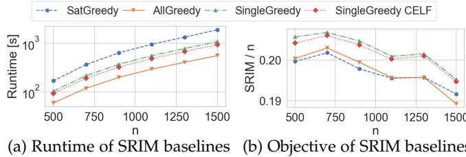
Fig. 3: SRIM on BA, p=0.4 , \mu=10 , W=0.3 , k=50 .
