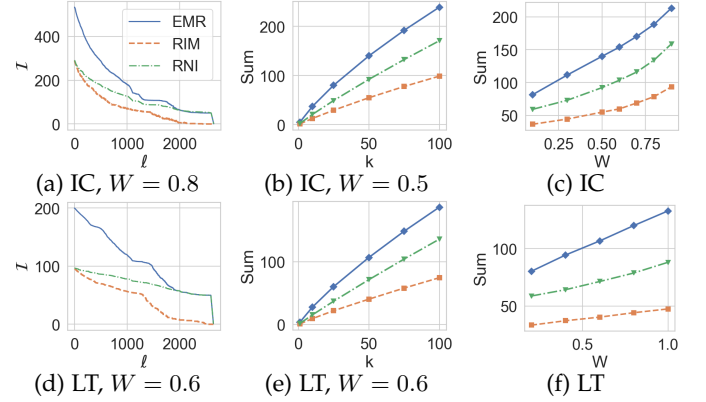
Fig. 4: Measures on Minnesota road network. k=50
