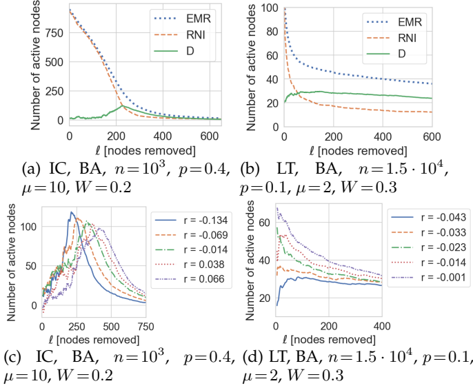
Fig. 11: Local maximum of D ; BA; k=5
