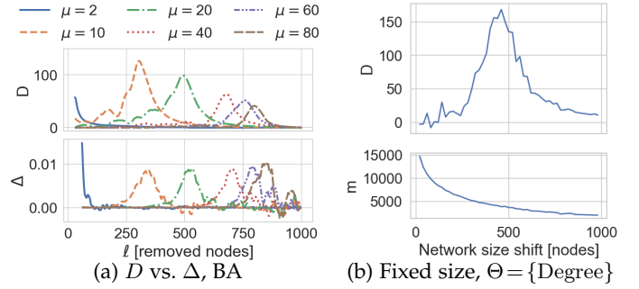
Fig. 12: Local maximum of D ; BA; n=1000 , p=0.4 , \mu=10 ; k=1
