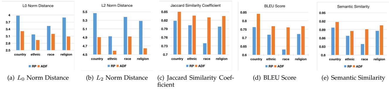
Fig. 8. Validity analysis.
