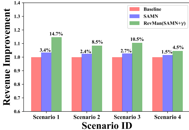
Figure 5: Offline evaluation in revenue improvement of RevMan. Compared with SAMN, RevMan achieves 11.3%, 6.1%, 7.8% and 3% revenue improvement in the four scenarios respectively.
