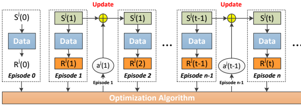
Figure 4: Workflow of discount estimator. It is initialized by a randomly chosen state S^j(0) . Then action a^j(t) is updated based on the environmental feedback of episode t and t-1 . The process ends when \sum_{\forall i,u} \Delta R_u^j(i) < \epsilon .
