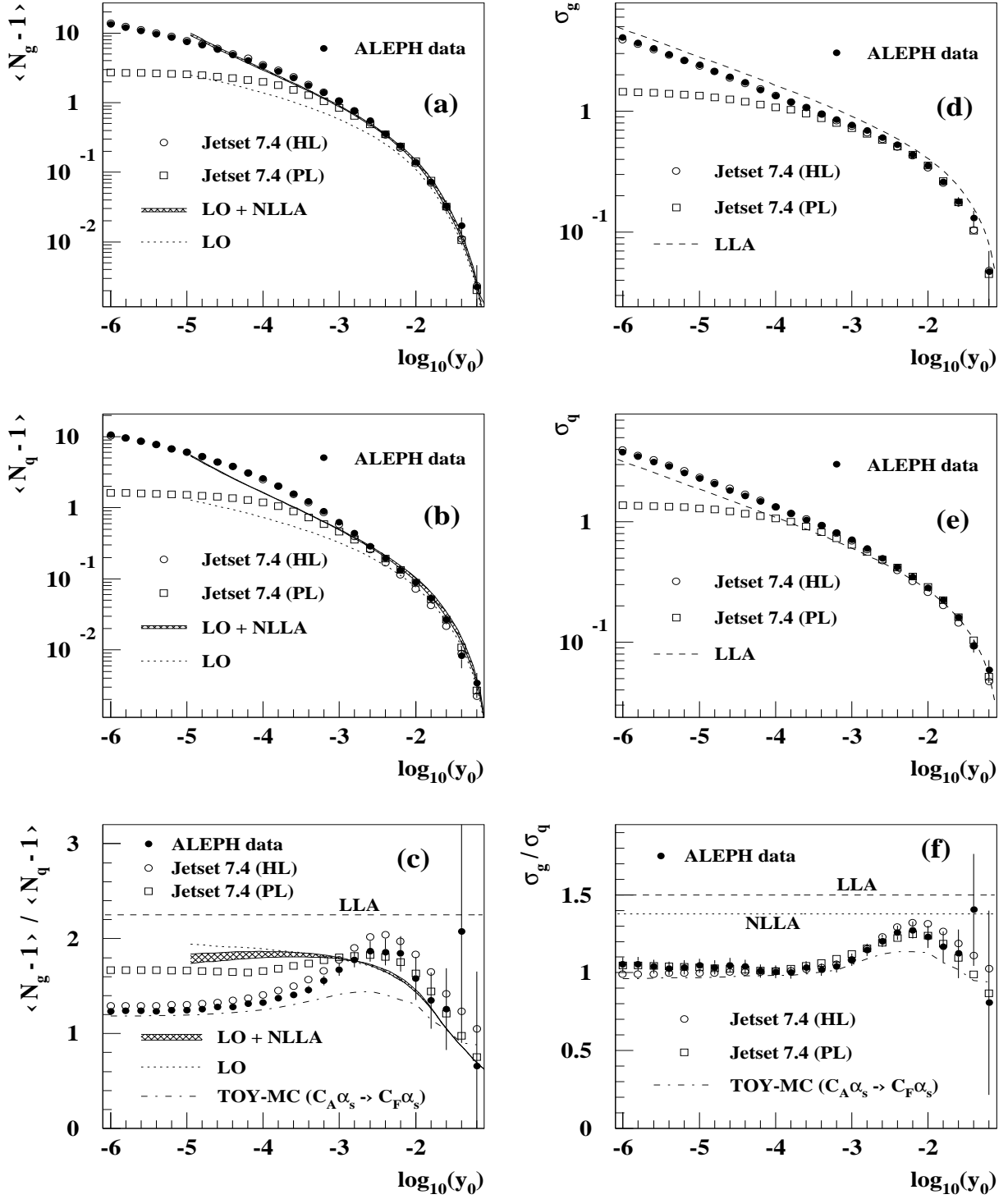
Figure 5: The mean (left-hand side) and the width (right-hand side) of the subjet multiplicity distribution are shown for gluon jets, quark jets and the ratio \frac{g_{luon}}{quark} as a function of the subjet resolution parameter y_0 . The full dots show the measurement and the open circles and squares represent the hadron and parton level from the JETSET MC (if the open circles are not visible in some of the plots they lie on top of the data points). The dashed-dotted line in the ratio plots shows the hadron level prediction of JETSET with C_A \alpha_s changed to C_F \alpha_s (see Section 5.1). The other lines show perturbative QCD predictions at various levels of precision (see text).
