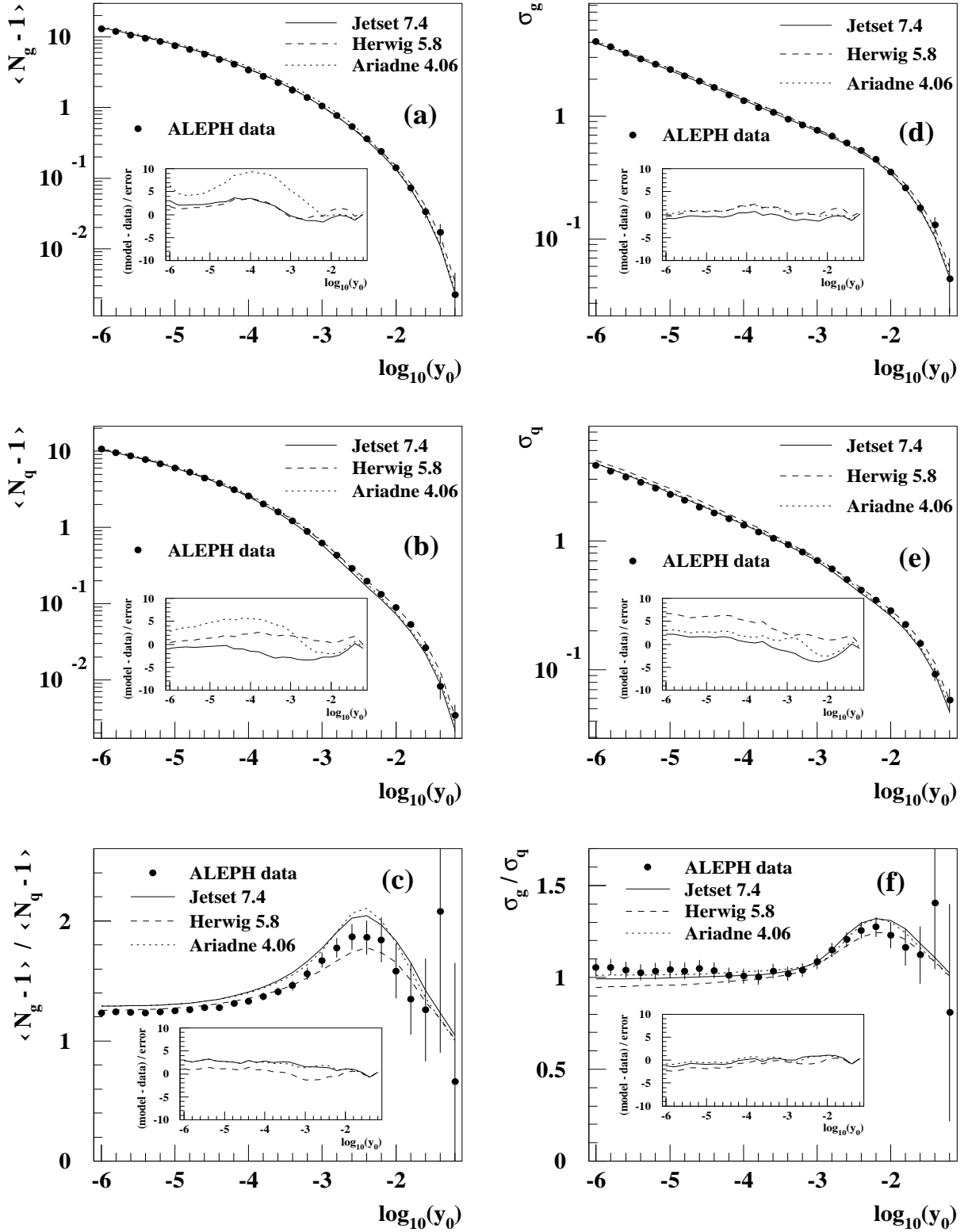
Figure 4: The mean (left-hand side) and the width (right-hand side) of the subjet multiplicity distribution are shown for gluon jets, quark jets and the ratio \frac{gluon}{quark} as a function of the subjet resolution parameter y_0 . The full dots show the measurement and the different lines represent the predictions of MC models. The inset plots show the deviations of the model predictions from the data divided by the total error. All plots apply to the whole interval of available jet energies.
