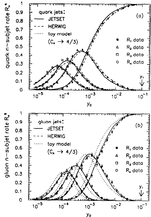
Fig. 5. Measured n -subjett rates R_n for (a) quark jets and (b) gluon jets (points) as a function of the subjett resolution parameter y_0 . Also shown are the predictions of various Monte Carlo models (curves).
