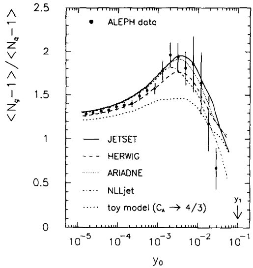
Fig. 3. Measured ratios of subjet multiplicities minus one \langle N_g - 1 \rangle / \langle N_q - 1 \rangle for gluon and quark jets (points) with the predictions of various Monte Carlo models (curves) as a function of the subjet resolution parameter y_0 .
