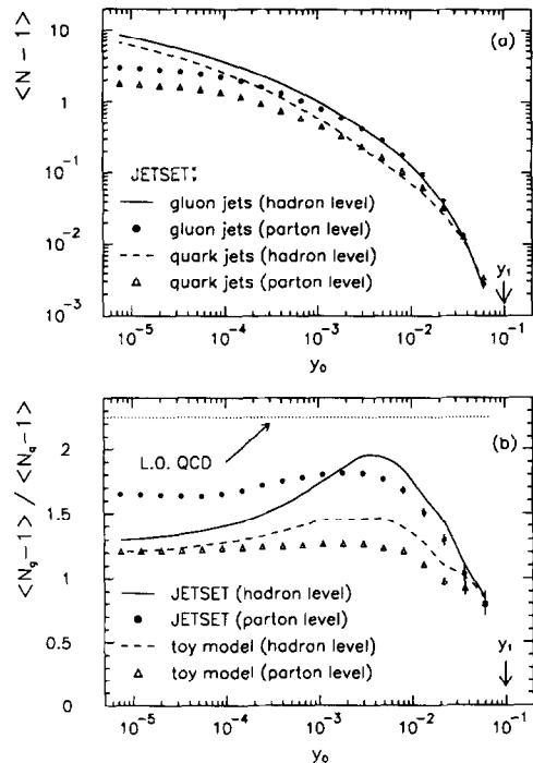
Fig. 4. (a) Mean subjet multiplicities for quark and gluon jets on both hadron and parton levels as predicted by the JETSET model. (b) The ratio of mean subjet multiplicities \langle N_g - 1 \rangle / \langle N_q - 1 \rangle obtained from JETSET and from a toy model in which the gluon's color charge C_A was reduced from 3 to 4/3. Also shown is the prediction of leading order QCD, C_A/C_F = 9/4 .
