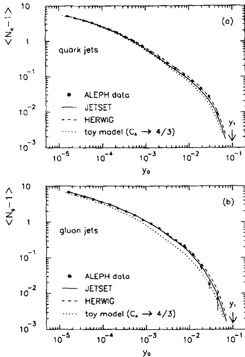
Fig. 2. Measured mean subjet multiplicity minus one (points) for (a) quark jets \langle N_q - 1 \rangle and (b) gluon jets \langle N_g - 1 \rangle as a function of the subjet resolution parameter y_0 . Also shown are the predictions of various Monte Carlo models (curves).
