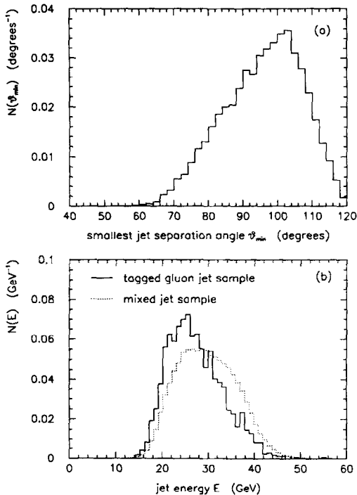
Fig. 1. (a) Distribution of the smallest separation angle between jets \theta_{min} in all three-jet events. (b) Distribution of jet energies in the tagged and mixed gluon samples. All distributions are normalized to unit area.
