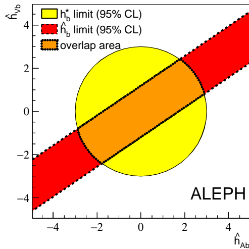
Figure 1: Combined results. The shaded areas depict the constraints of the measurements on the couplings \hat{h}_{Ab} and \hat{h}_{Vb} .
