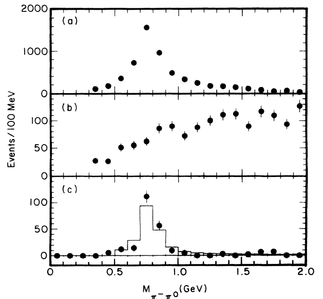
FIG. 9. (a) The \pi^0 \pi^- invariant mass spectrum for a B^- \rightarrow D^0 \rho^- Monte Carlo simulation. (b) The \pi^0 \pi^- invariant mass spectrum B^- \rightarrow D^0(\pi^-\pi^0)_{\text{NR}} Monte Carlo simulation. (c) The \pi^0 \pi^- invariant mass spectrum for the B^- \rightarrow D^0 \pi^0 \pi^- mode in data.
