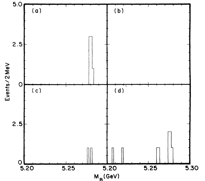
FIG. 23. Beam-constrained mass for (a) B^- \rightarrow \psi' K^- , (b) \bar{B}^0 \rightarrow \psi' \bar{K}^0 , (c) B^- \rightarrow \psi' \bar{K}^{*-} , and (d) \bar{B}^0 \rightarrow \psi' K^{*0} .
