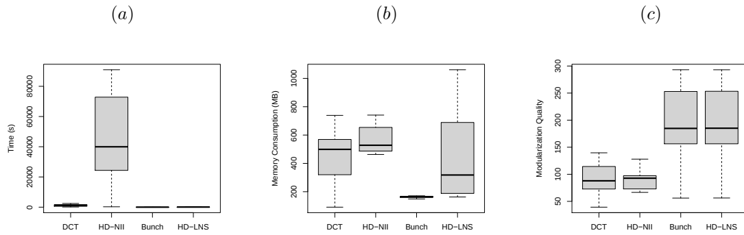
Fig. 2. Performance comparison of SMC tools. (a) Compares TS, (b) compares MMC, and (c) compares MQ. We removed the outliers in the boxplots.
