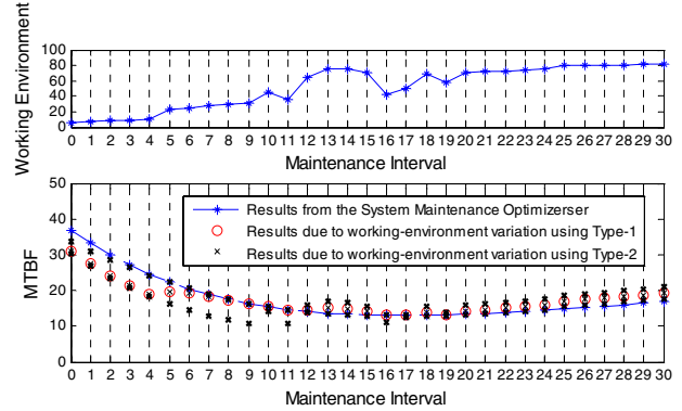
Fig. 8 Updated MTBF Due to Working-environment Variation
