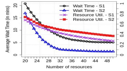
Figure 16: Waiting Time vs. Resource Utilization with T_D=5\text{mins} ( C=1 )
