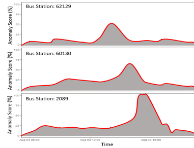
Figure 19: Spatial Evolution of Anomaly Score (NDR)
