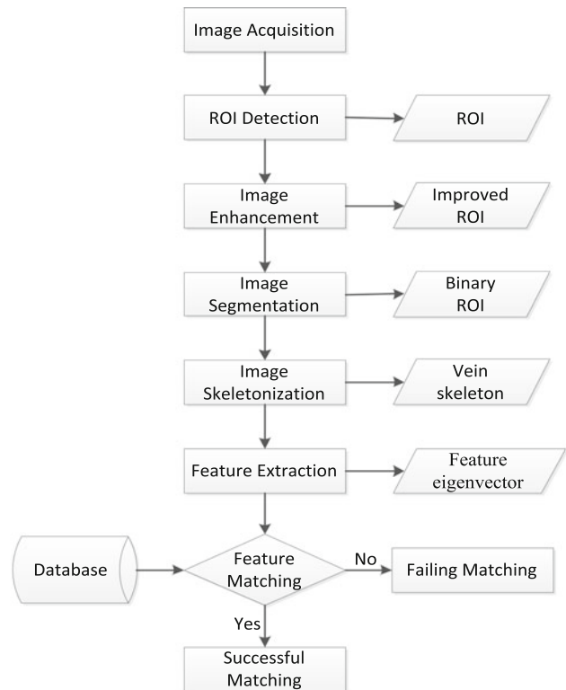
Fig. 1 Process of palm vein identification
