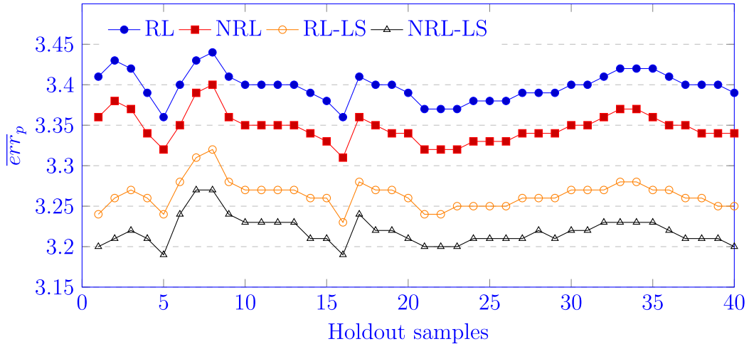
Fig. 7. Average of the test error values over holdout samples.
